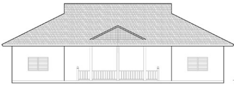
RESOURCE CENTER ELEVATION
