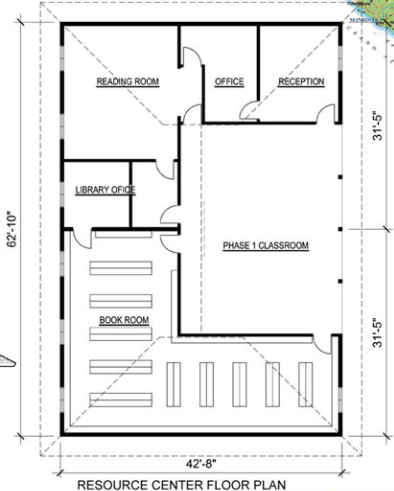
RESOURCE CENTER FLOOR PLAN
